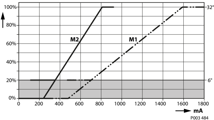
Displacement (%) versus Input Command (mA)
