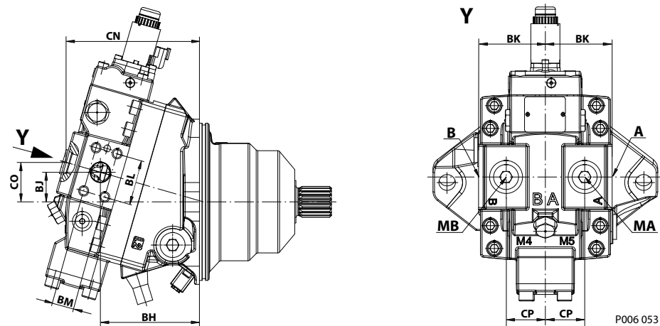
Radial ports
