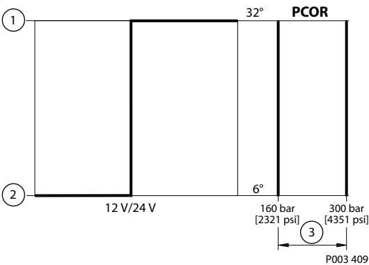
Displacement versus PCOR pressure
